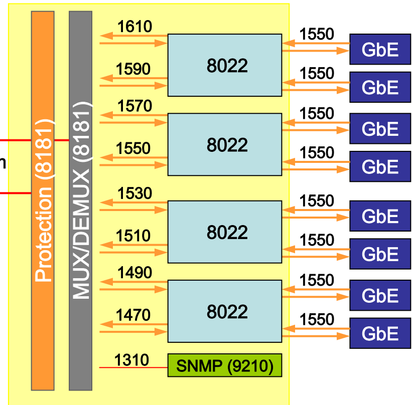
SML2000 Chassis
